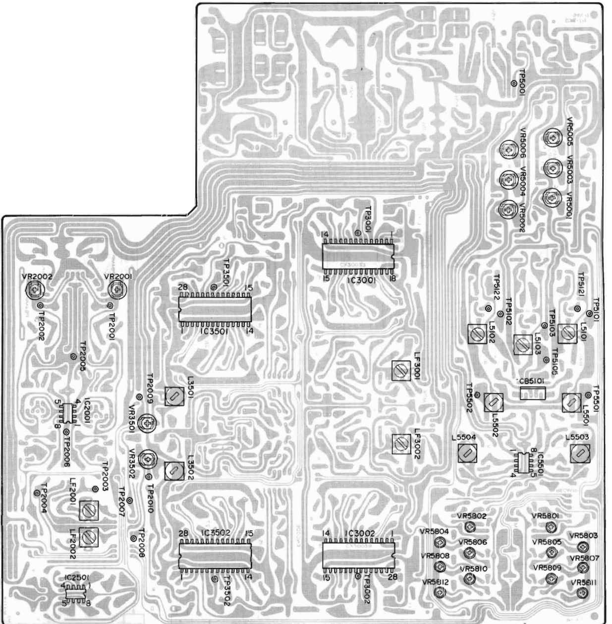
Mother P.C. Board
