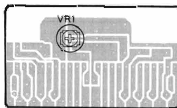
Wire Assembly P.C. Board
